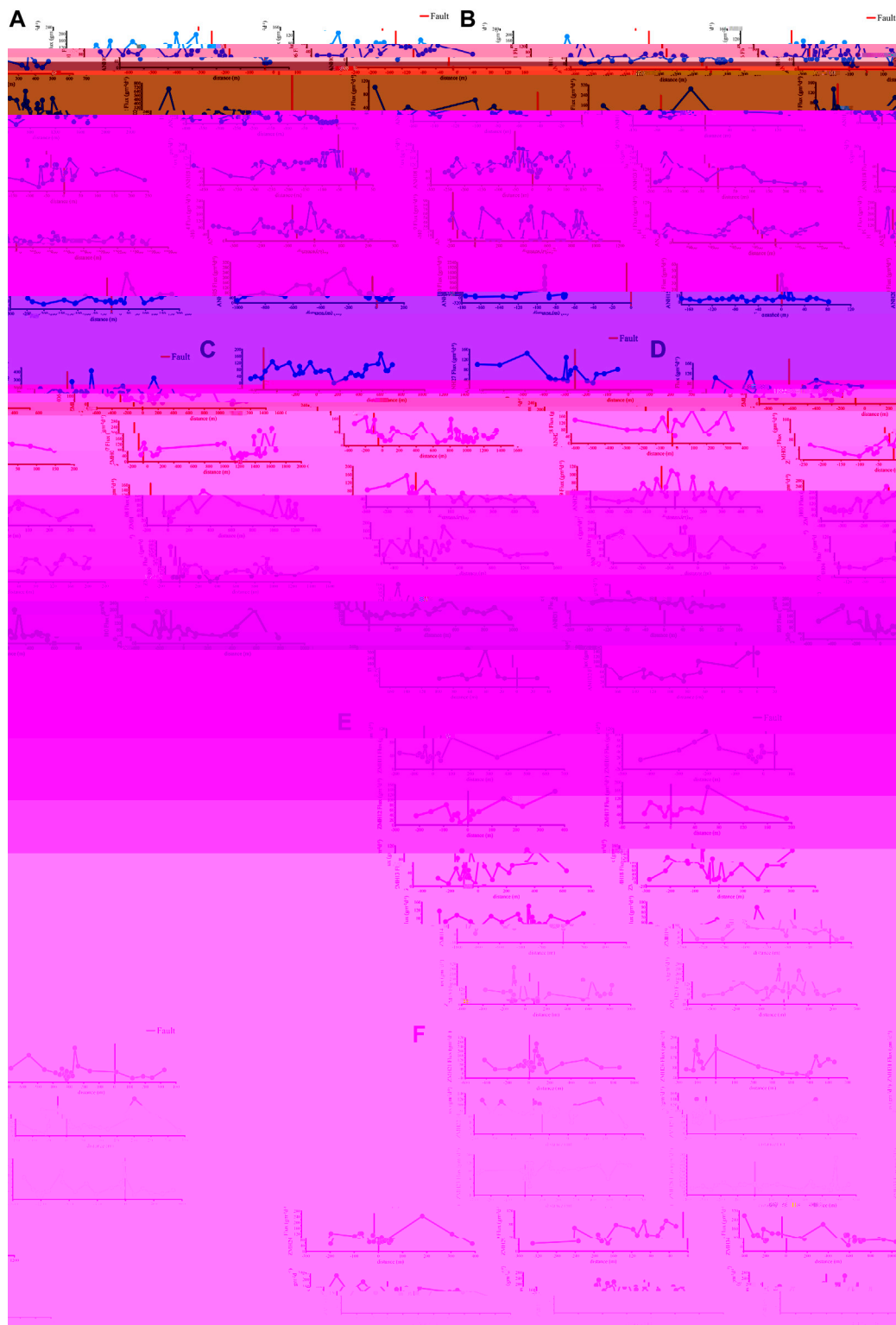
FIGURE 5 Profiles of CO 2 concentration and δ 13 C-CO 2 in the study area. (A) Profile of CO 2 concentration and δ 13 C-CO 2 in the study area. (B) Profile of CO 2 concentration and δ 13 C-CO 2 in the study area. (C) Profile of CO 2 concentration and δ 13 C-CO 2 in the study area. (D) Profile of CO 2 concentration and δ 13 C-CO 2 in the study area. (E) Profile of CO 2 concentration and δ 13 C-CO 2 in the study area. (F) Profile of CO 2 concentration and δ 13 C-CO 2 in the study area.
